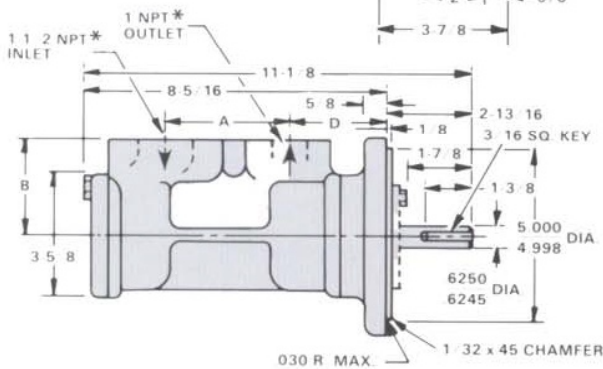
C3EIC- INTEGRAL FLANGE MOUNT-NO SEAL
