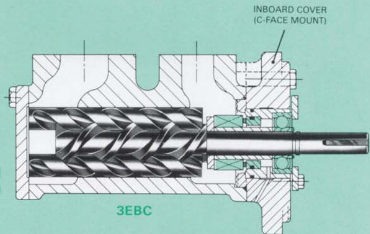
Flange Mount with Mechanical Seal and Ball Bearing
