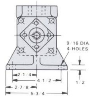
TYPE C3E * F FOOT MOUNTED
