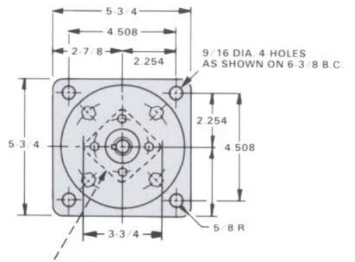
TYPES C3E * "C" FLANGE MOUNTED
